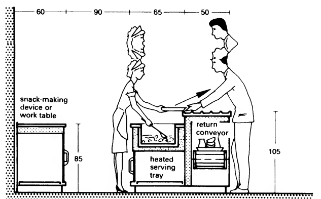
9 Cafeteria: meal servery → 8
